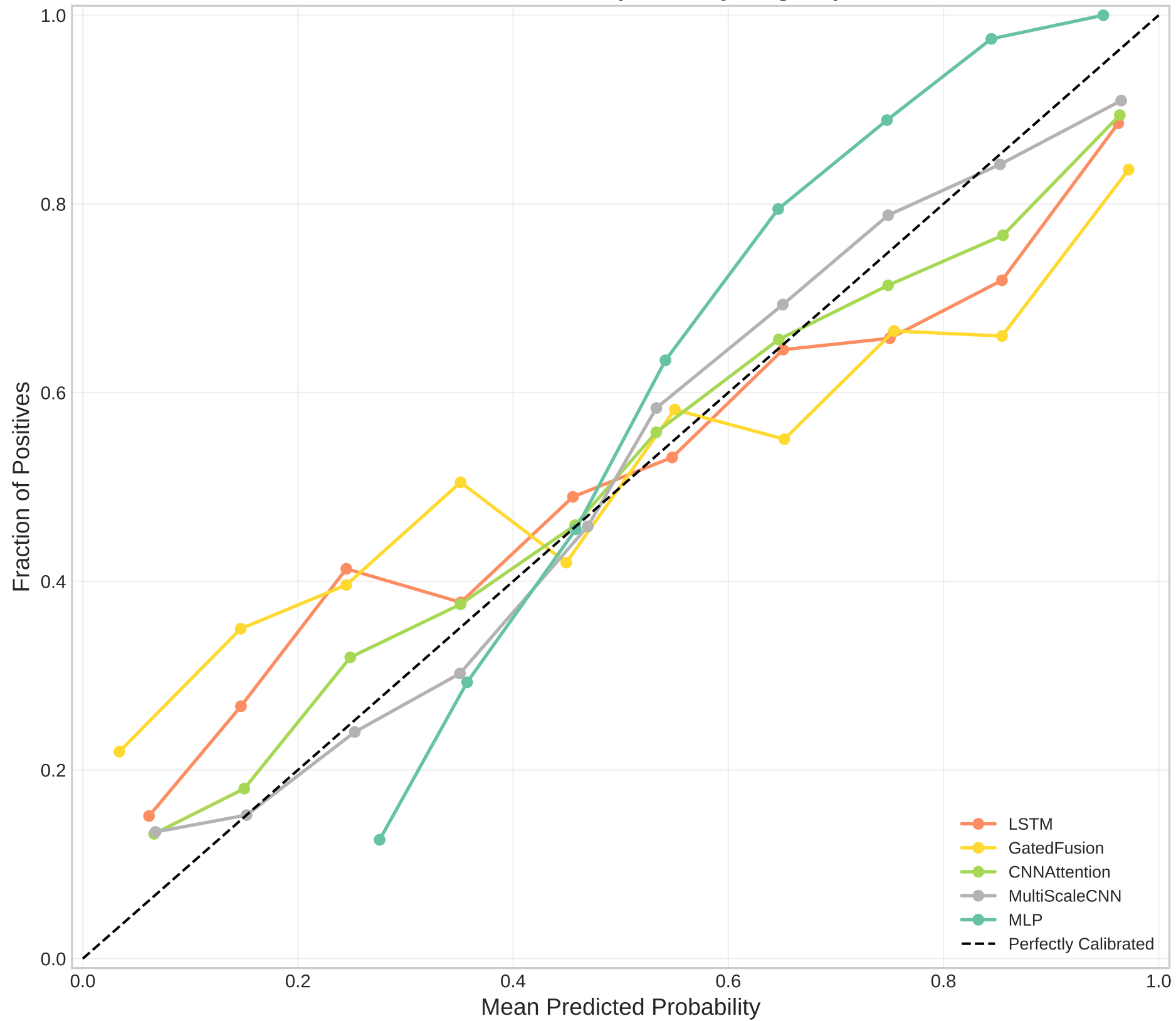
Calibration Curves (Reliability Diagram)
